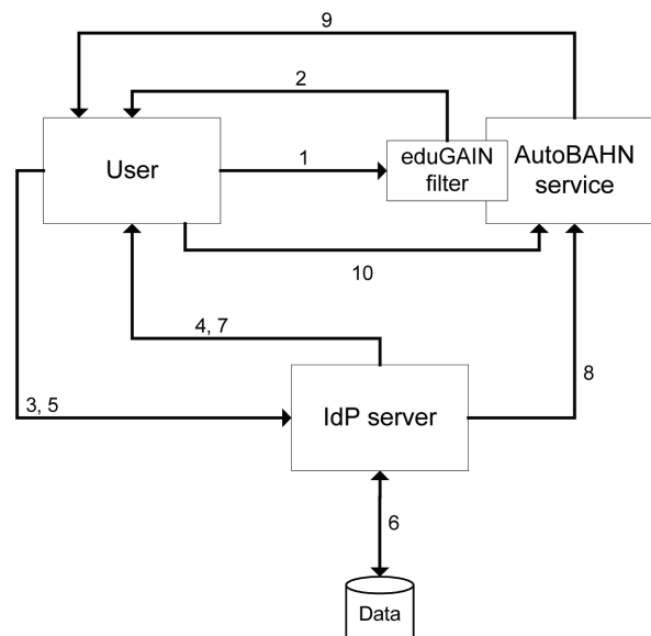
Figure 4. AutoBAHN Single-Sign On authentication procedure
