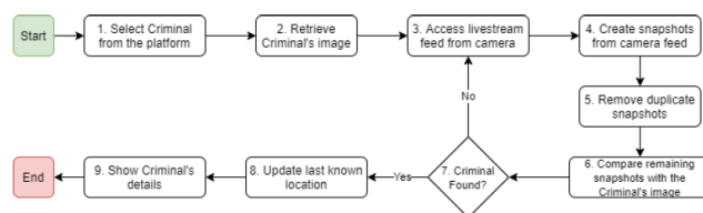
Fig. 1. The live feed facial recognition approach.
