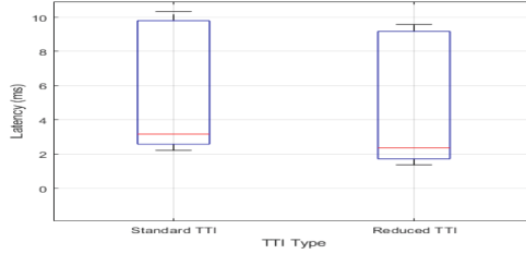
Fig. 2. Box Plot of Latency for Standard and Reduced TTI
