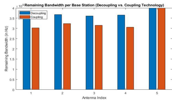
Fig. 6. Bandwidth Consumption for 724 UEs.
