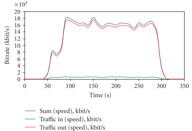
FIGURE 9: Bitrate versus Time for G@L Server.
